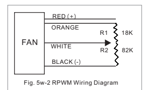
Fig. 5w-2 RPWM Wiring Diagram
